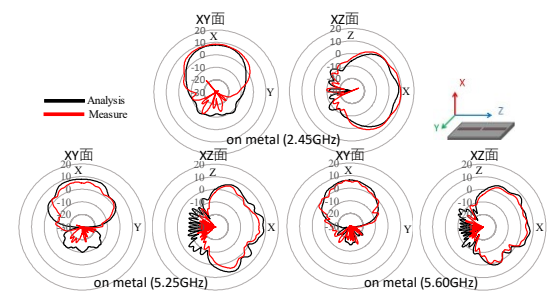
Fig. 8. Radiation patterns on a metal plate.
