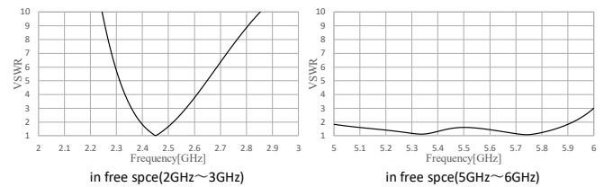
Fig. 2. VSWR characteristics of a parallel arrangement model.
