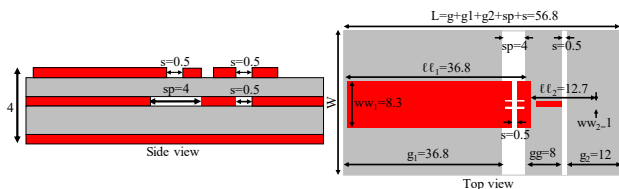
Fig. 5. Structure of a MACKEY type T.
