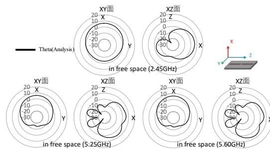
Fig. 3. Radiation patterns of a parallel arrangement model.
