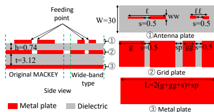
Fig. 1. Structure of a parallel arrangement model.
